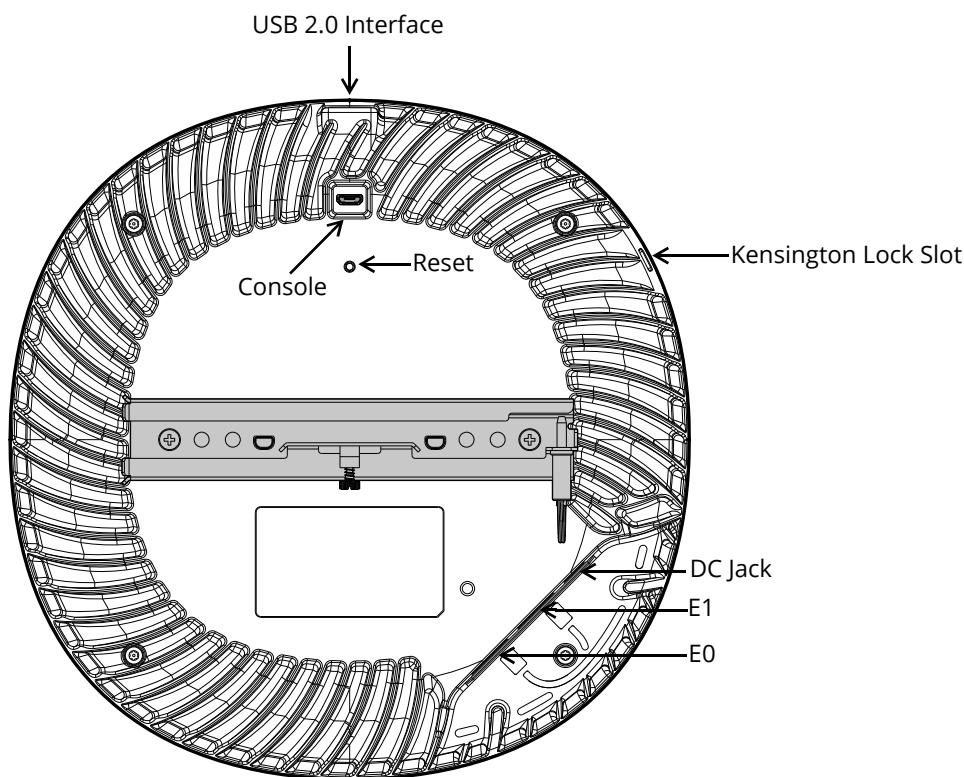
Figure 2 AP-635 Rear View
