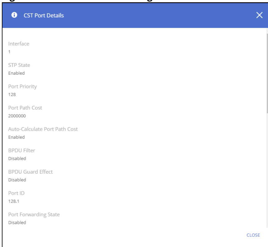
Figure 77. CST Port Details Page
