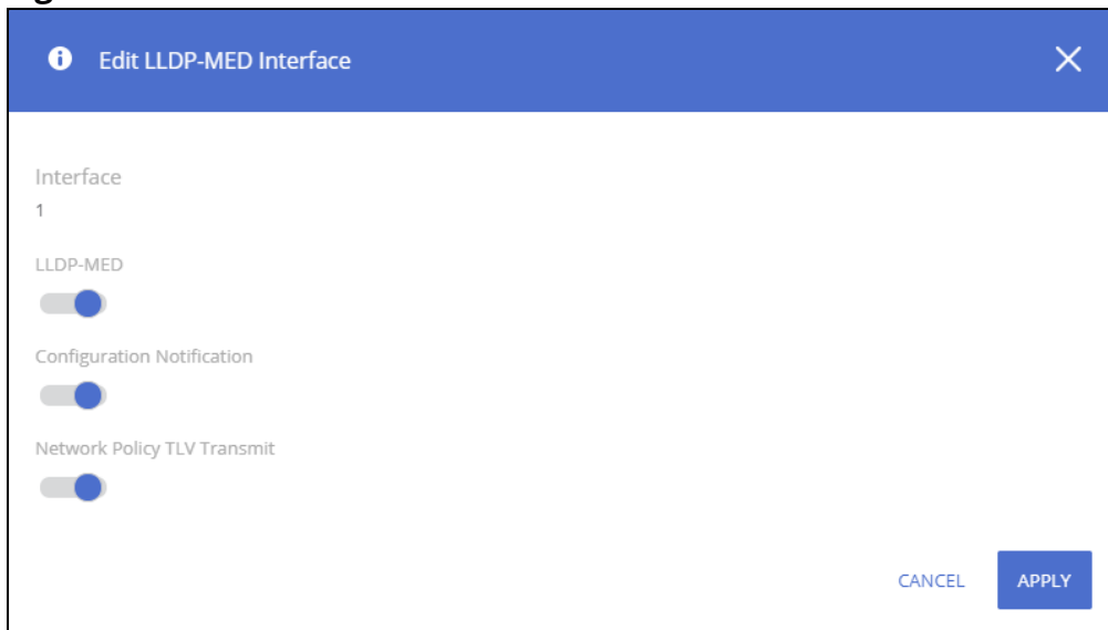
Figure 105. Edit LLDP-MED Interface
