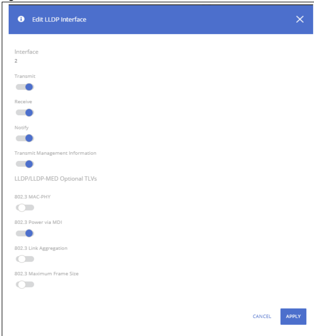
Figure 97. Edit LLDP Interface
