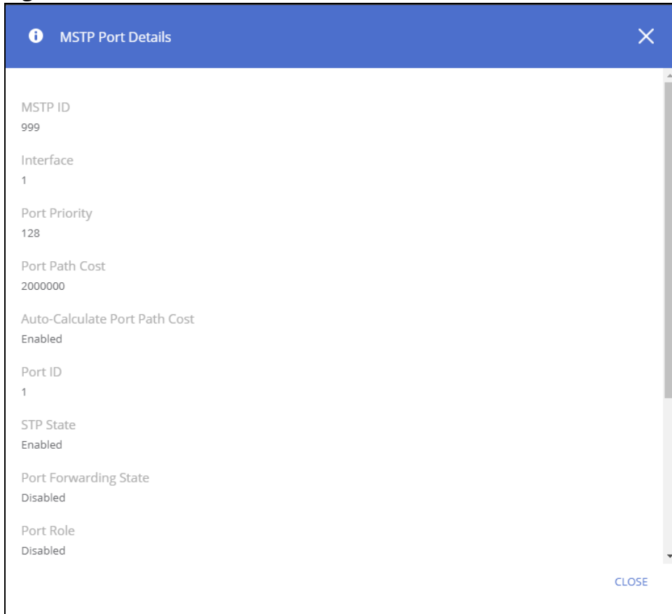
Figure 82. MSTP Port Details
