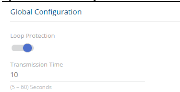
Figure 39. Global Configuration
